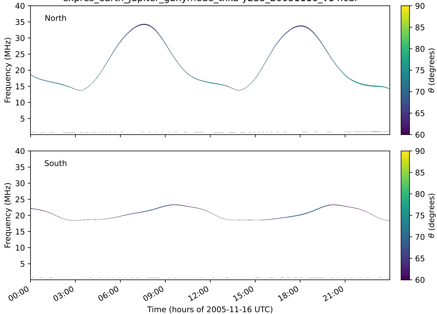
expres_earth_jupiter_ganymede_txka-y235_20051116_v14.cdf
