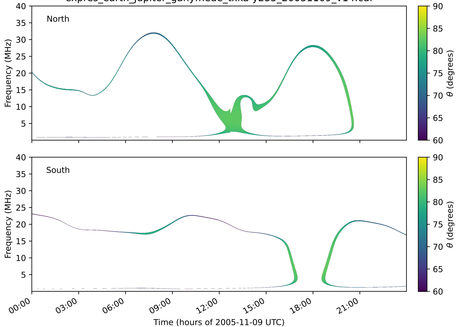
expres_earth_jupiter_ganymede_txka-y235_20051109_v14.cdf
