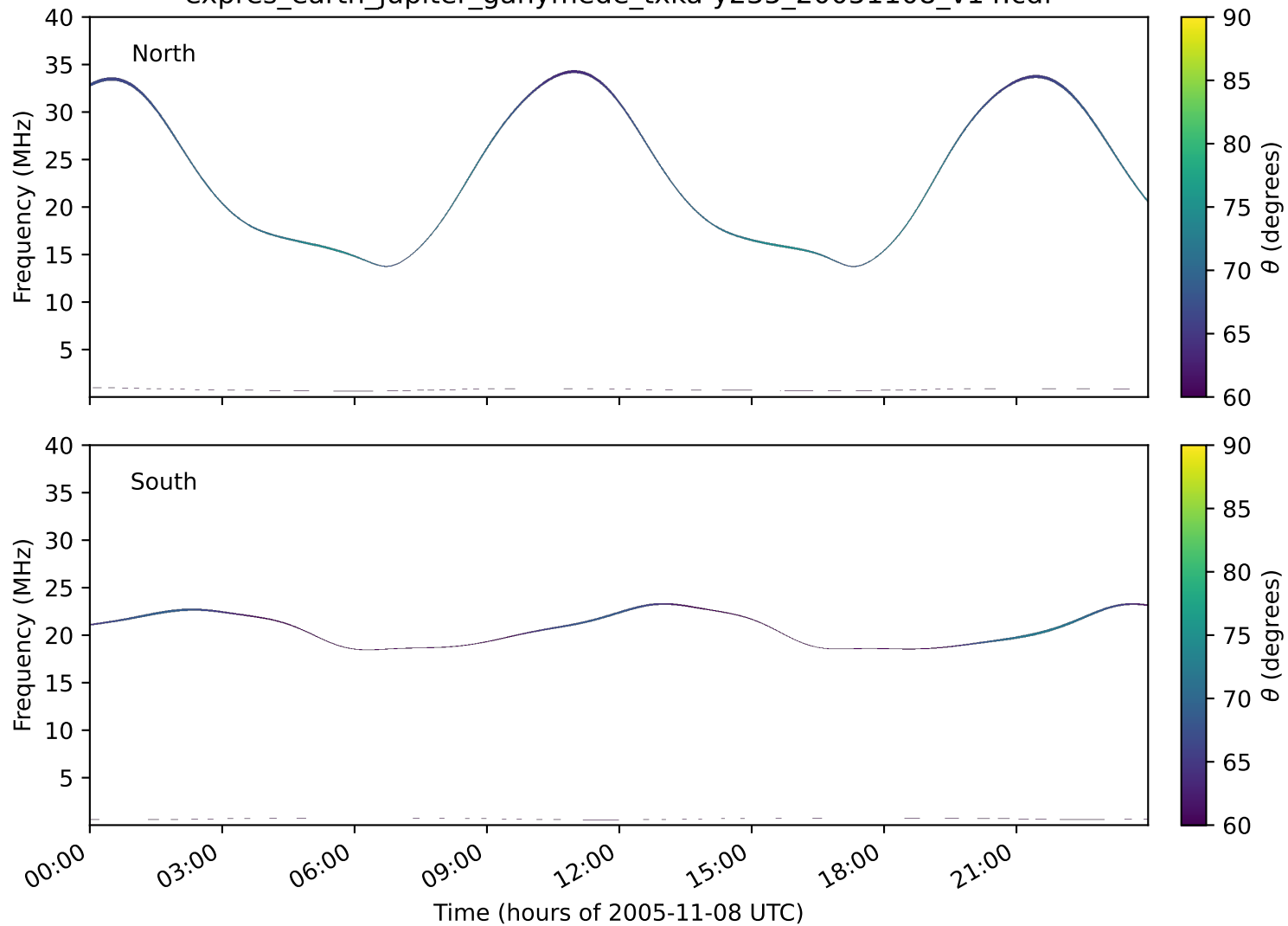
expres_earth_jupiter_ganymede_txka-y235_20051108_v14.cdf
