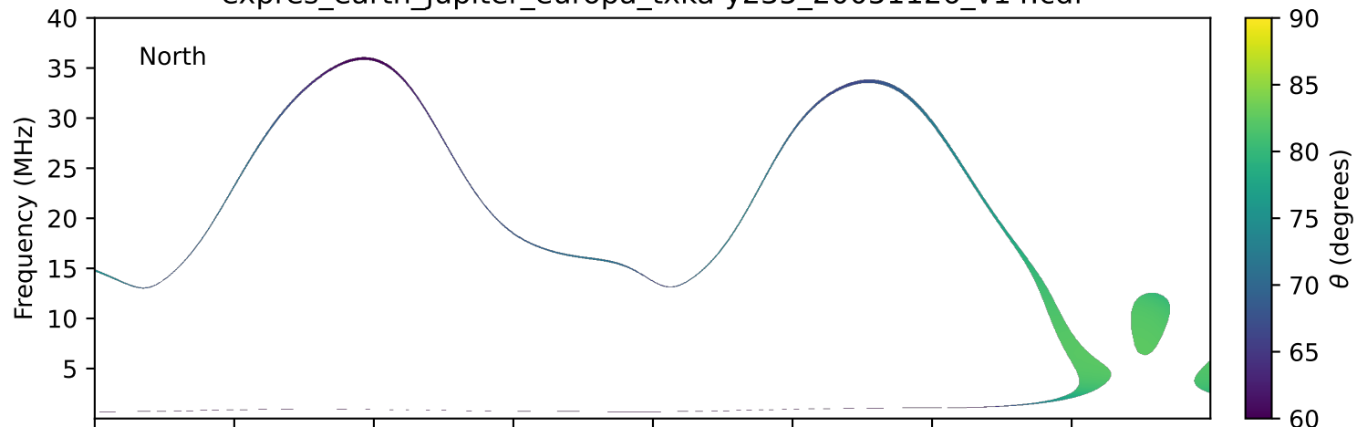
expres_earth_jupiter_europa_txka-y235_20051126_v14.cdf
