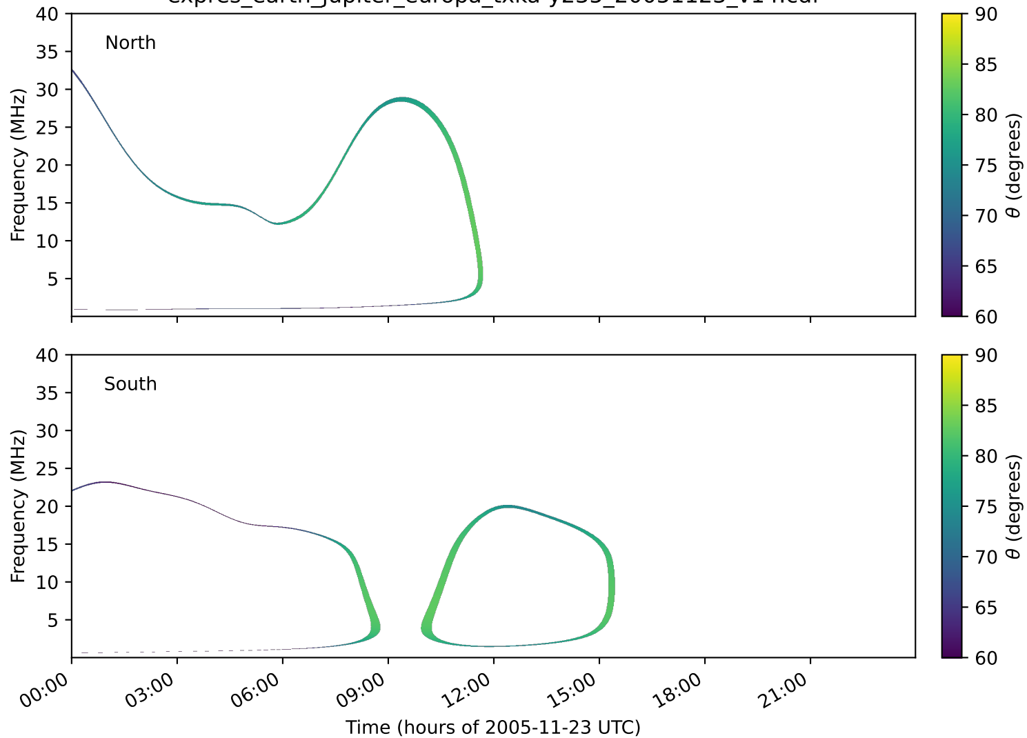
expres_earth_jupiter_europa_txka-y235_20051123_v14.cdf
