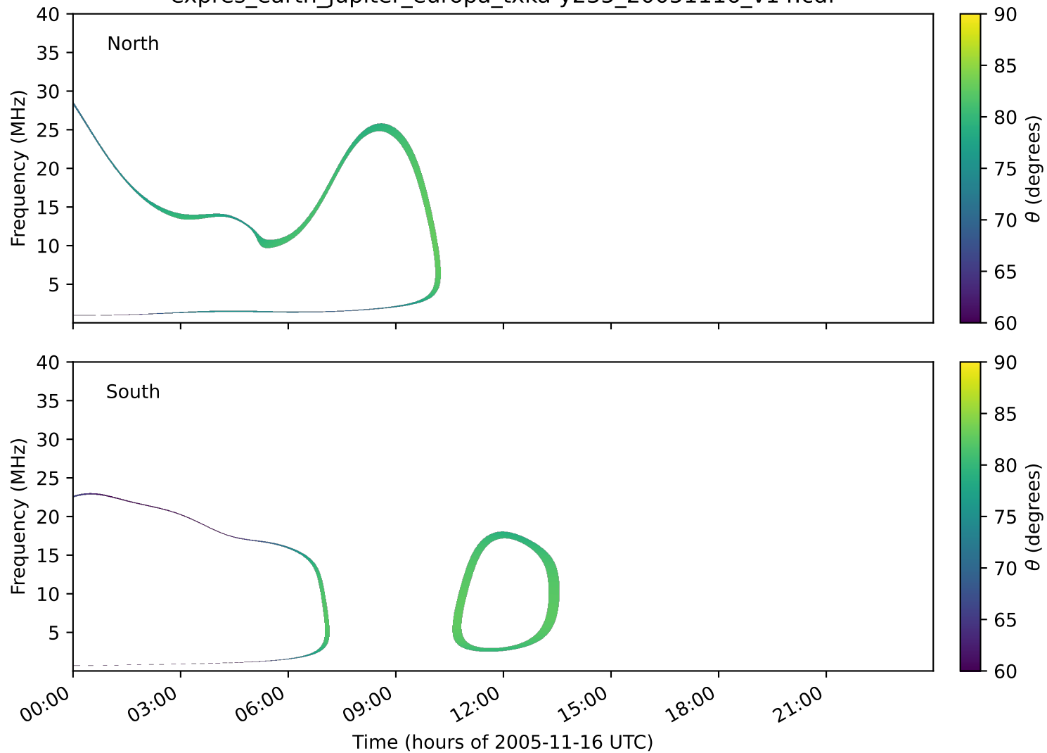
expres_earth_jupiter_europa_txka-y235_20051116_v14.cdf
