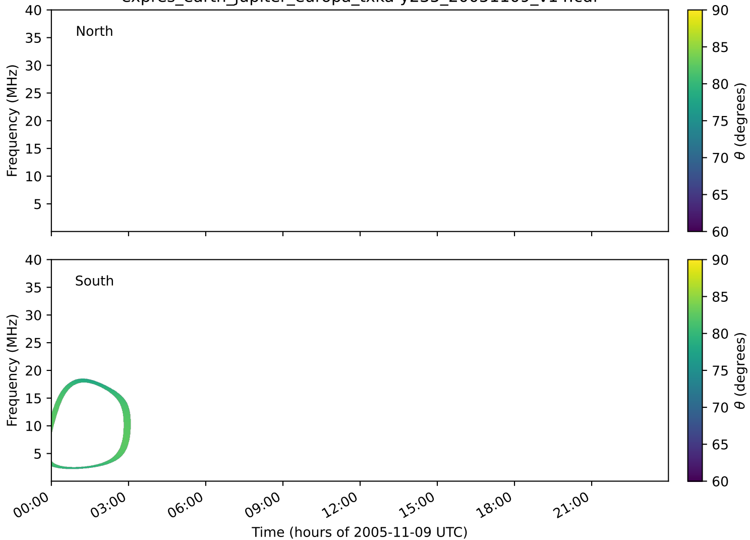
expres_earth_jupiter_europa_txka-y235_20051109_v14.cdf
