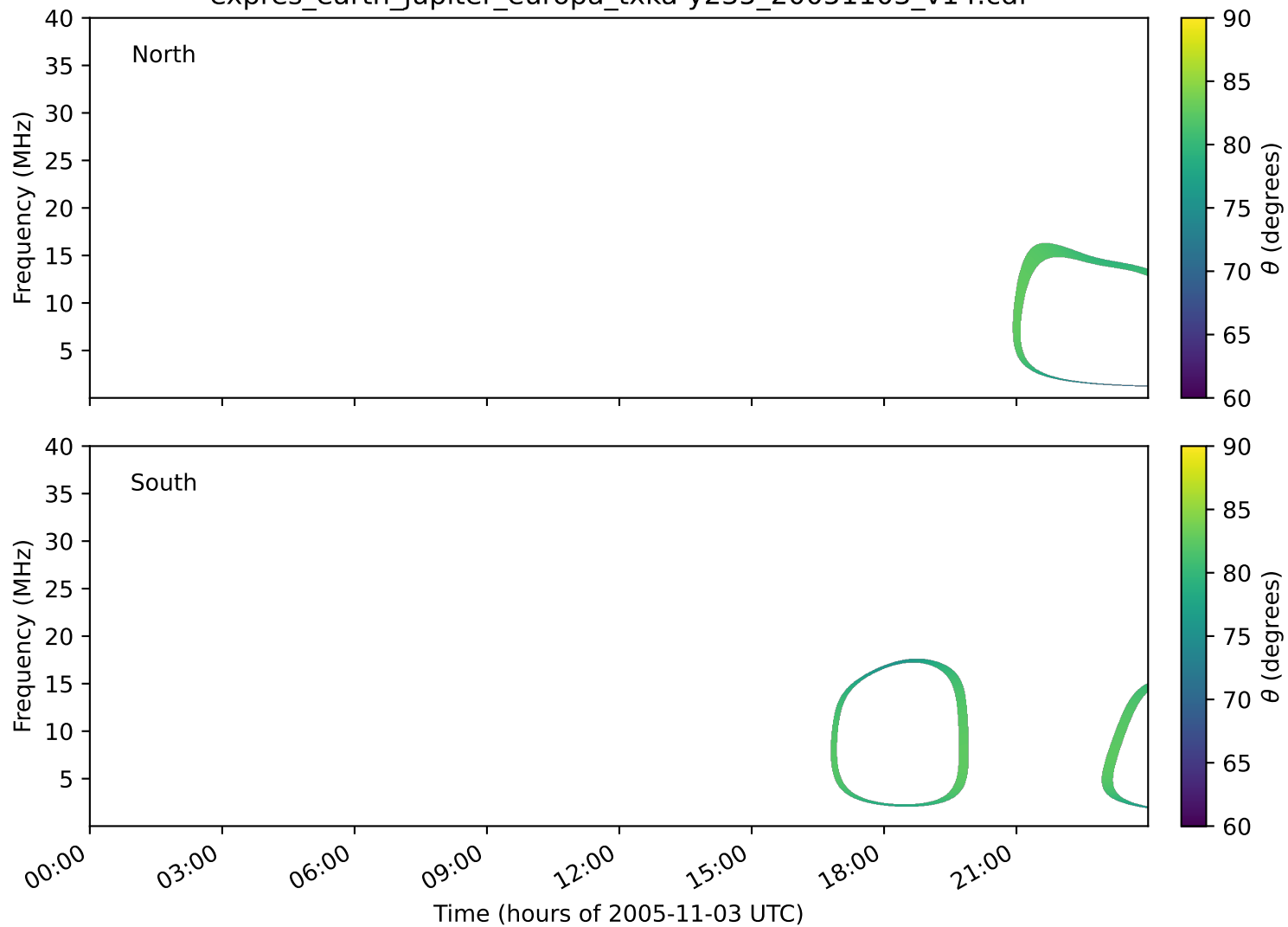
expres_earth_jupiter_europa_txka-y235_20051103_v14.cdf
