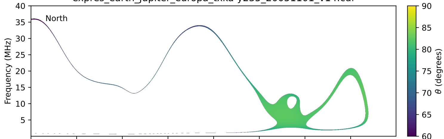
expres_earth_jupiter_europa_txka-y235_20051101_v14.cdf
