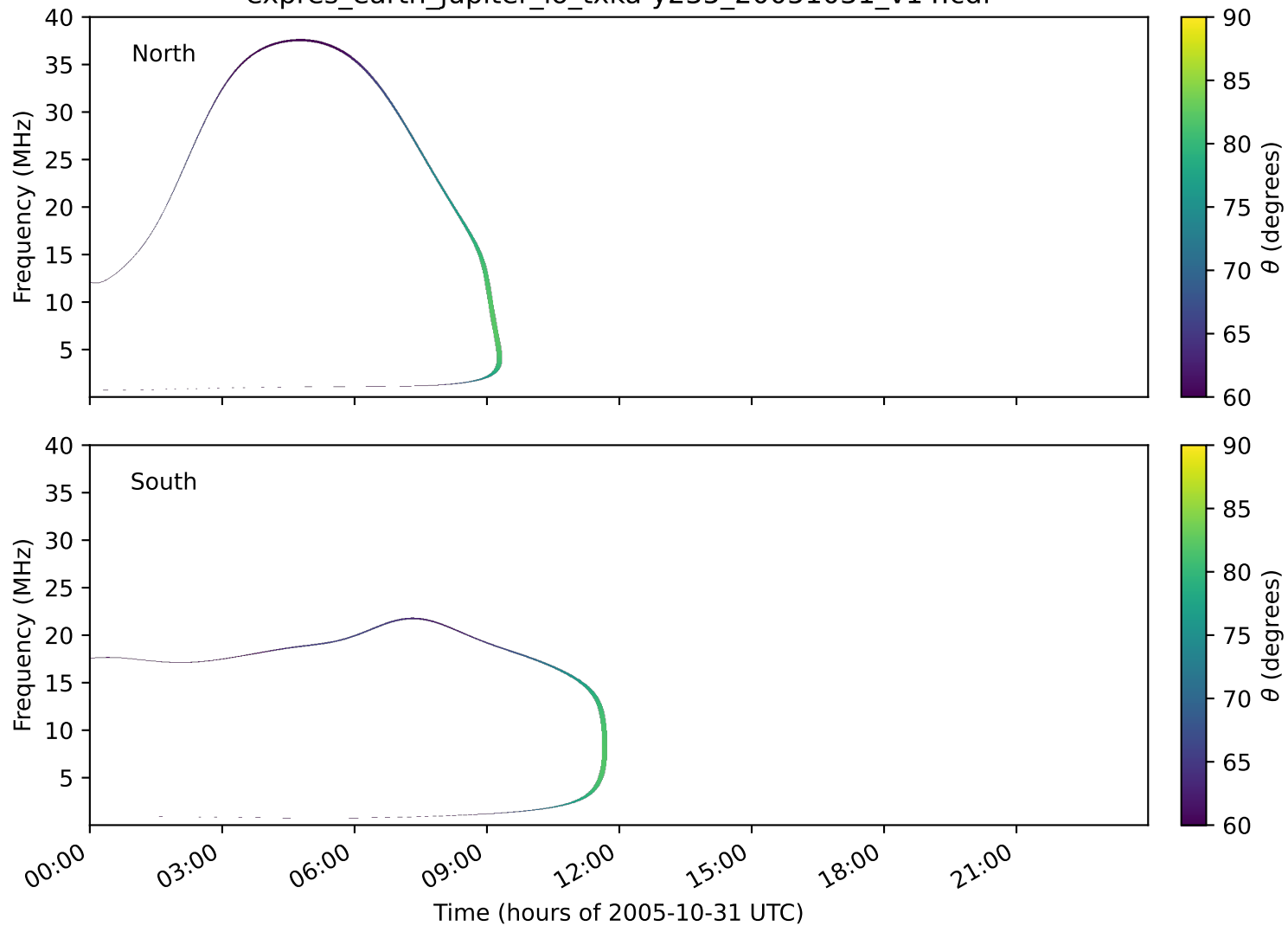
expres_earth_jupiter_io_txka-y235_20051031_v14.cdf
