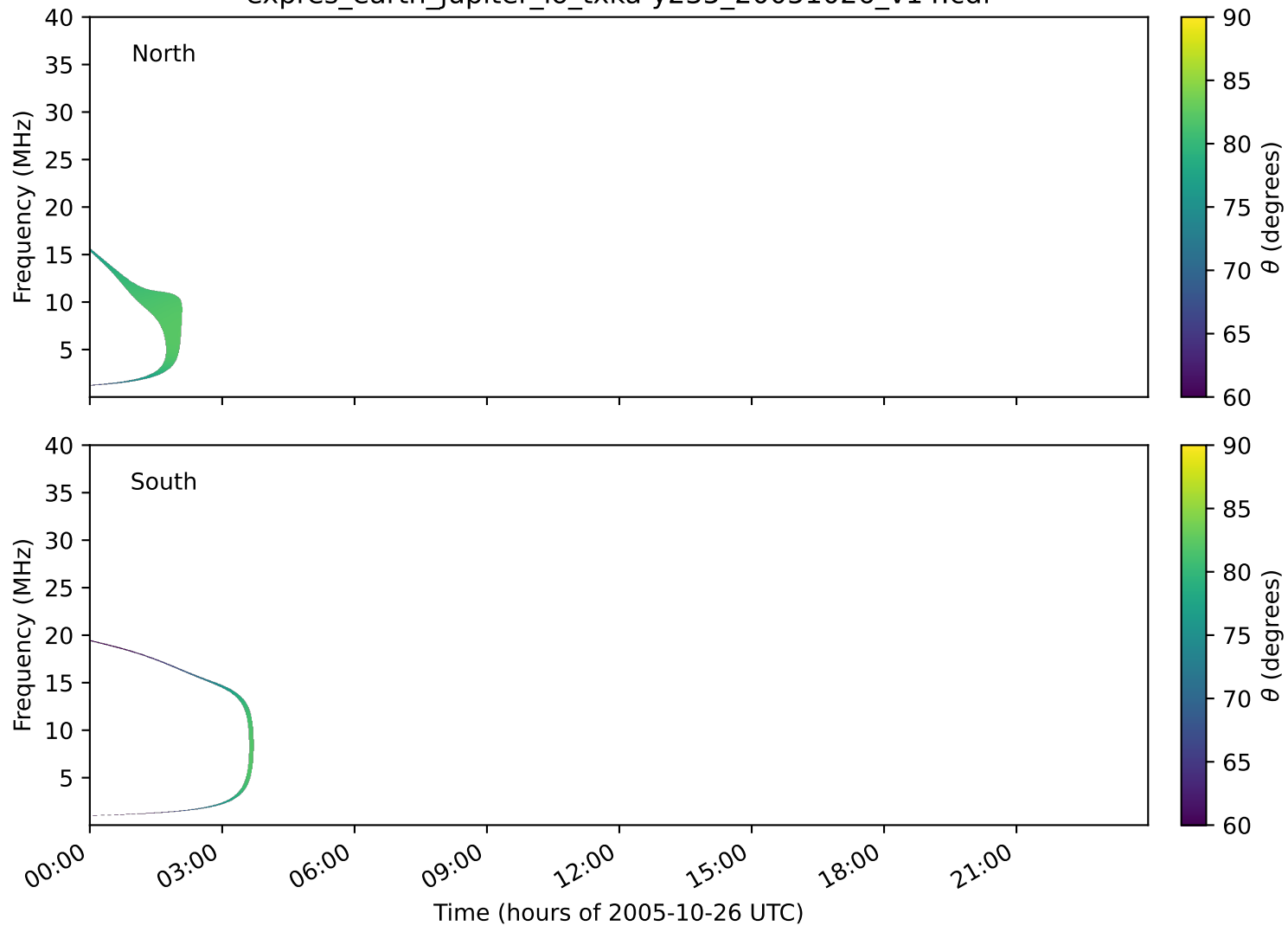
expres_earth_jupiter_io_txka-y235_20051026_v14.cdf
