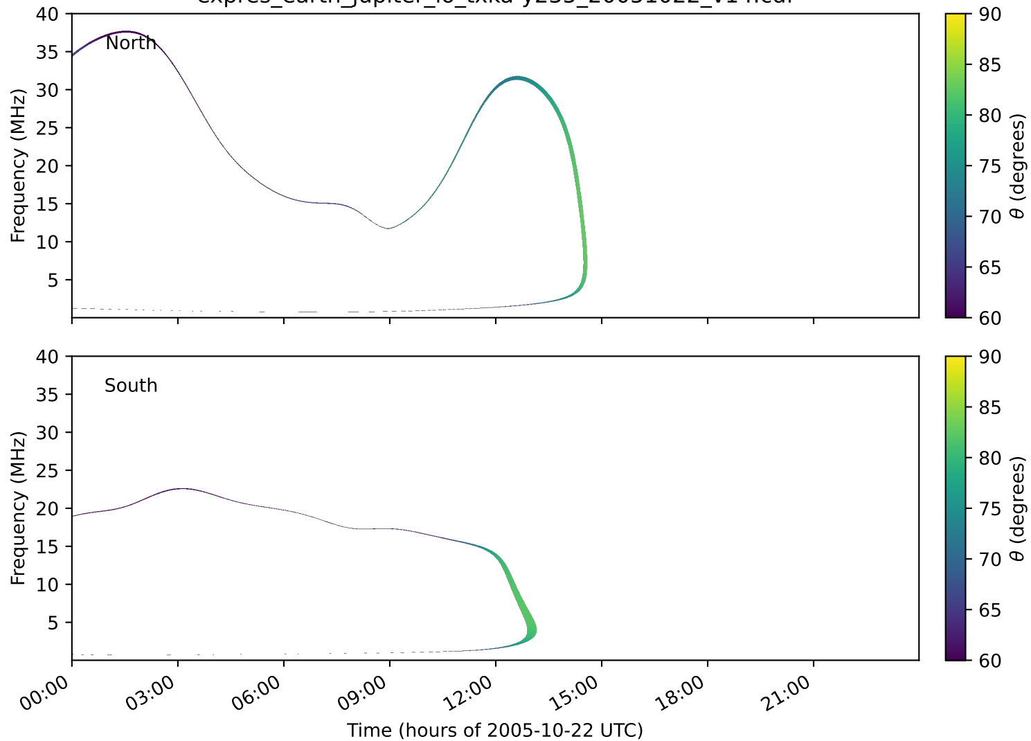
expres_earth_jupiter_io_txka-y235_20051022_v14.cdf
