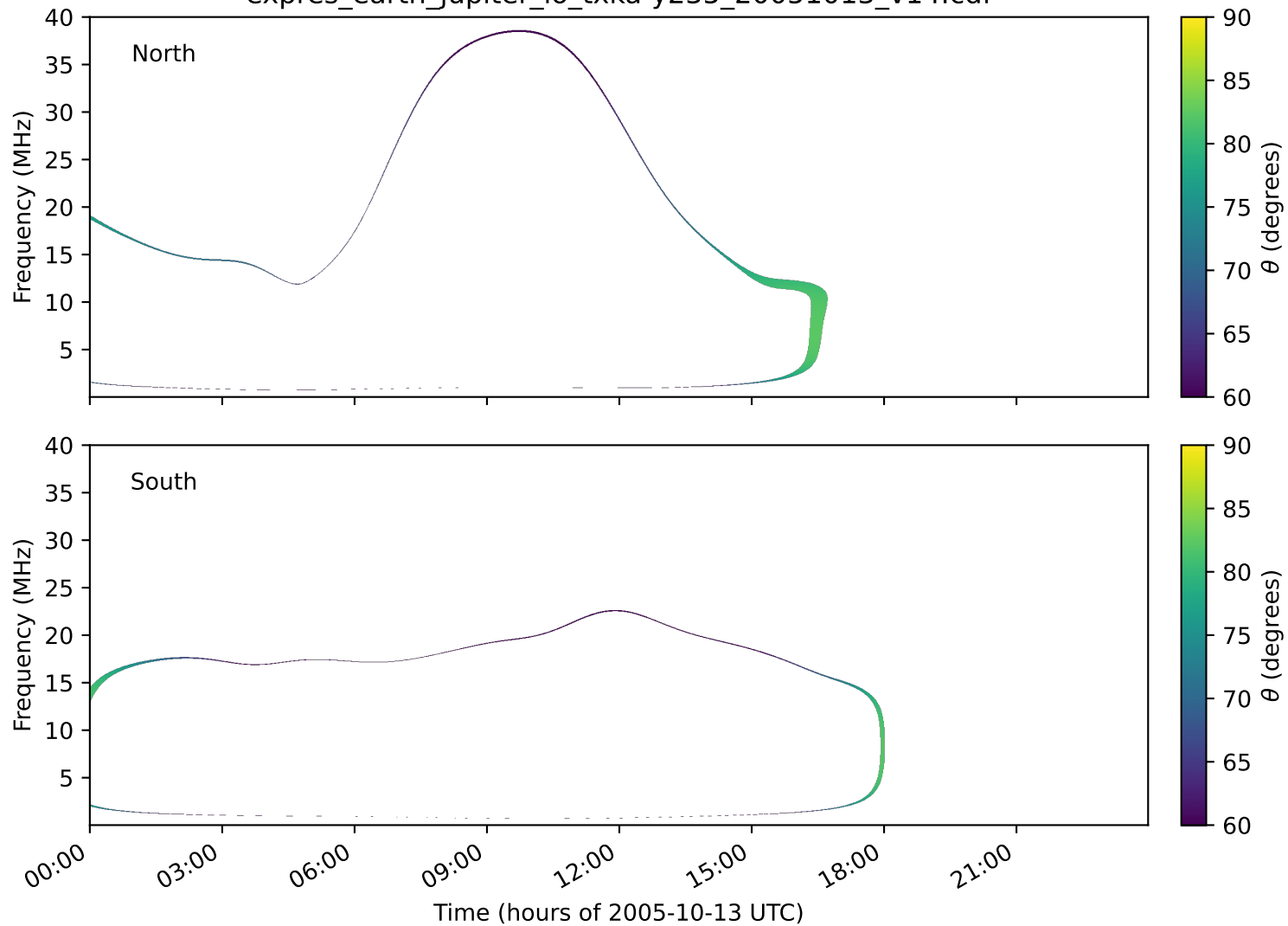
expres_earth_jupiter_io_txka-y235_20051013_v14.cdf
