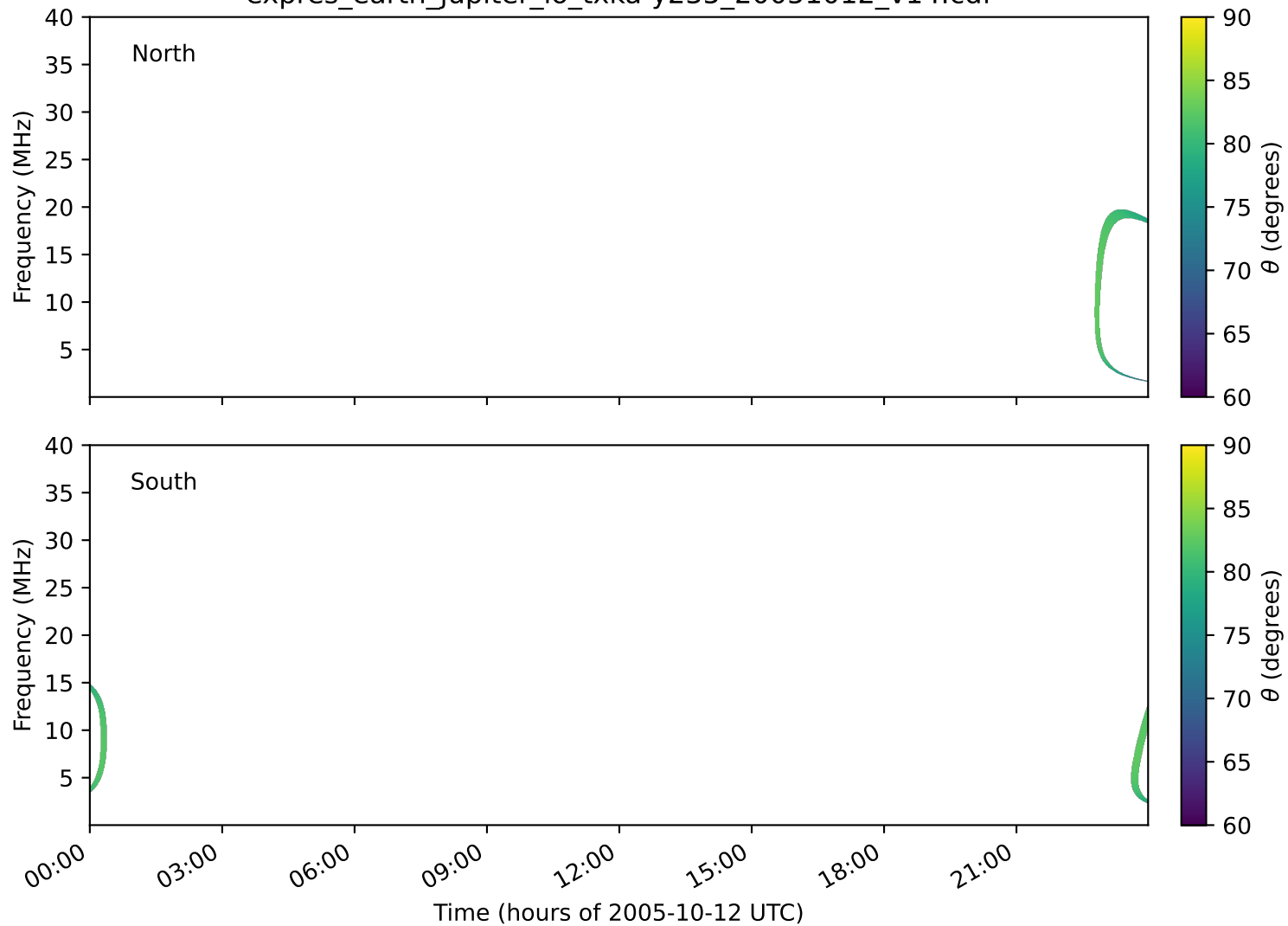
expres_earth_jupiter_io_txka-y235_20051012_v14.cdf
