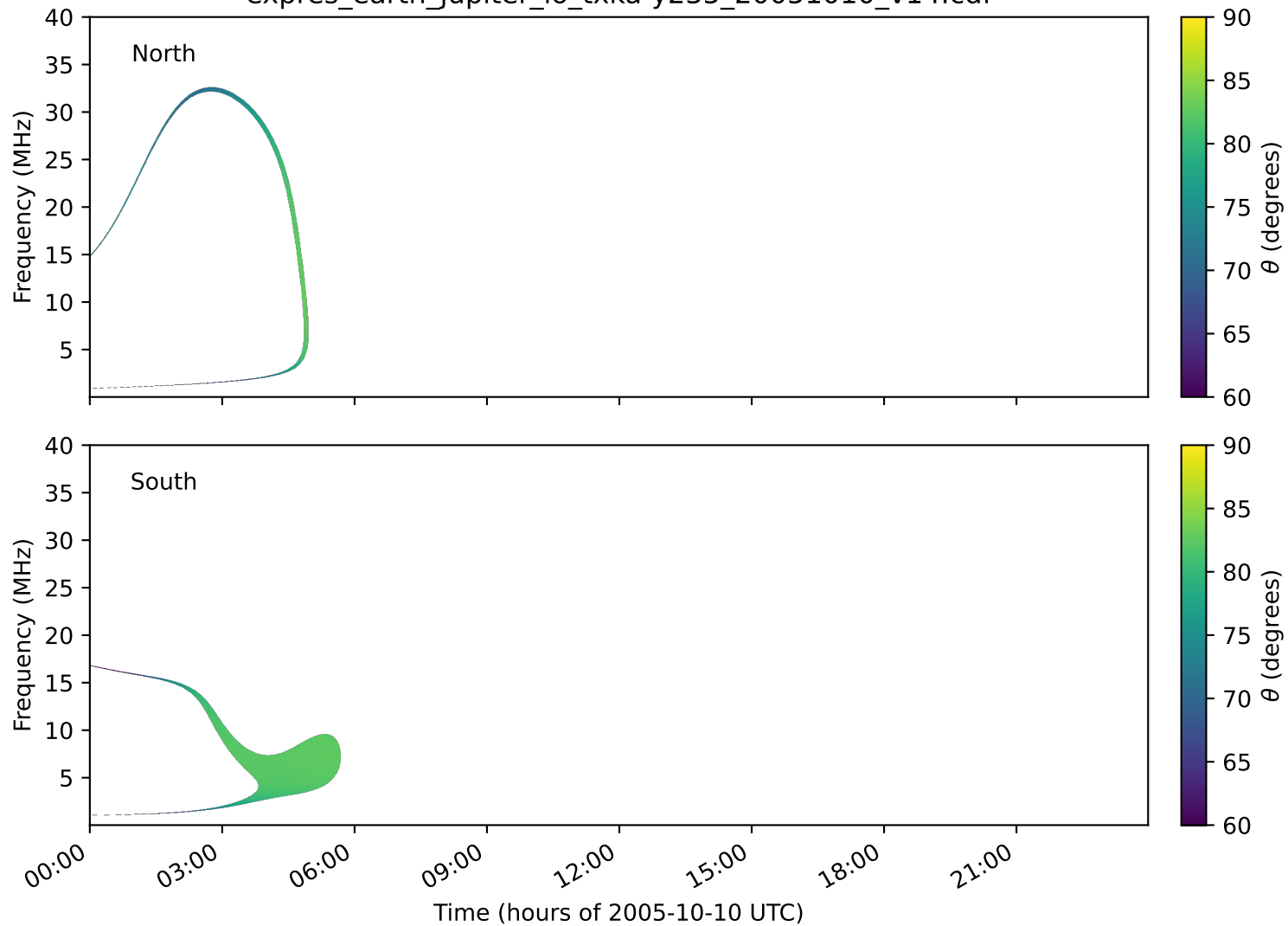
expres_earth_jupiter_io_txka-y235_20051010_v14.cdf
