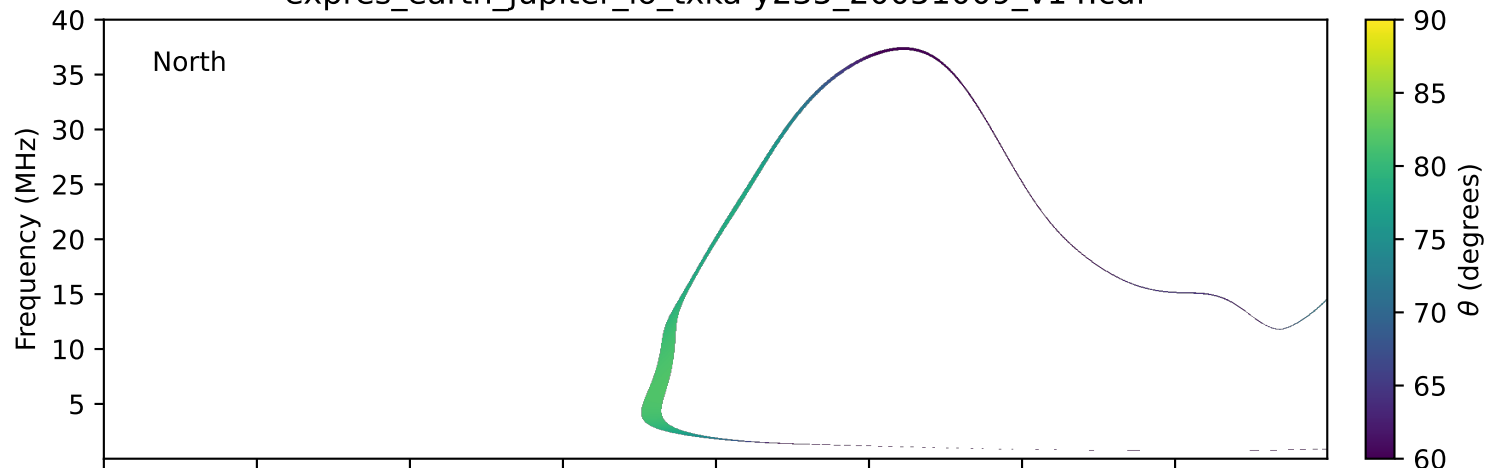
expres_earth_jupiter_io_txka-y235_20051009_v14.cdf
