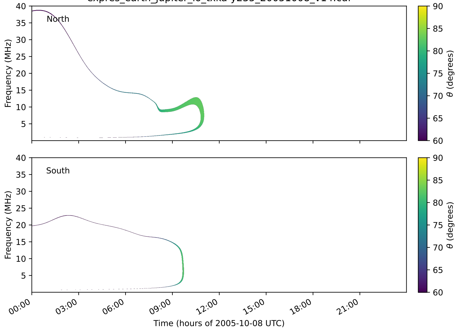
expres_earth_jupiter_io_txka-y235_20051008_v14.cdf
