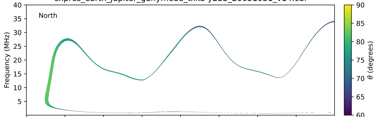
expres_earth_jupiter_ganymede_txka-y235_20051031_v14.cdf
