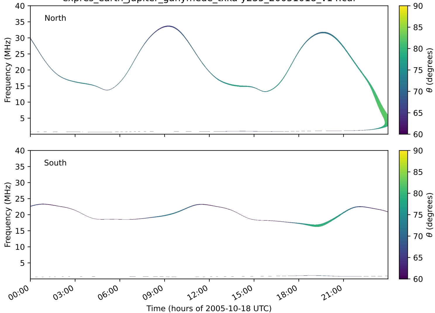
expres_earth_jupiter_ganymede_txka-y235_20051018_v14.cdf
