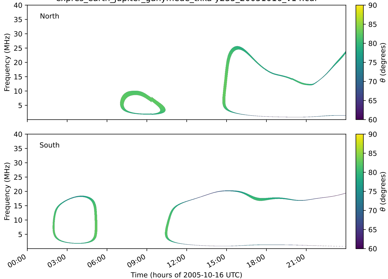
expres_earth_jupiter_ganymede_txka-y235_20051016_v14.cdf
