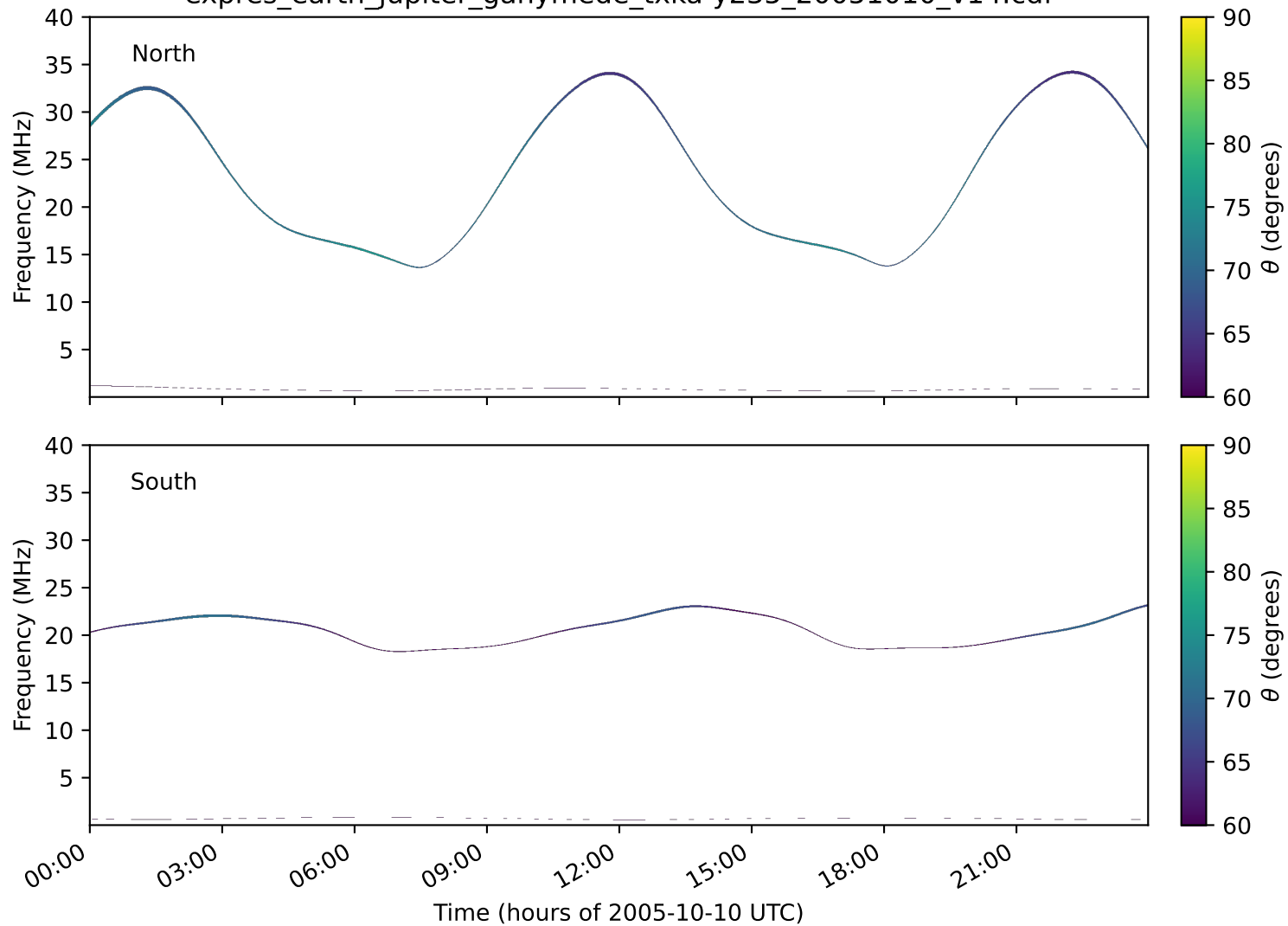
expres_earth_jupiter_ganymede_txka-y235_20051010_v14.cdf
