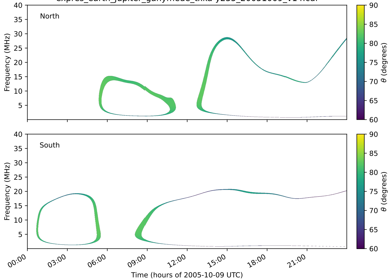
expres_earth_jupiter_ganymede_txka-y235_20051009_v14.cdf
