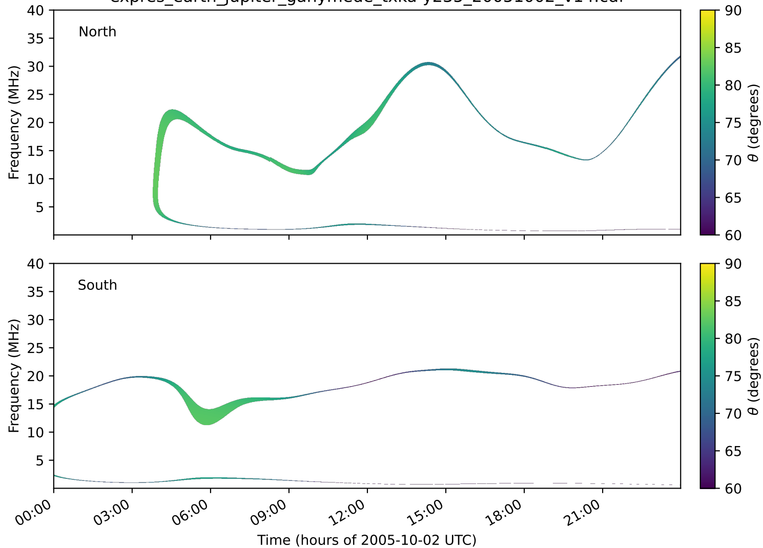
expres_earth_jupiter_ganymede_txka-y235_20051002_v14.cdf
