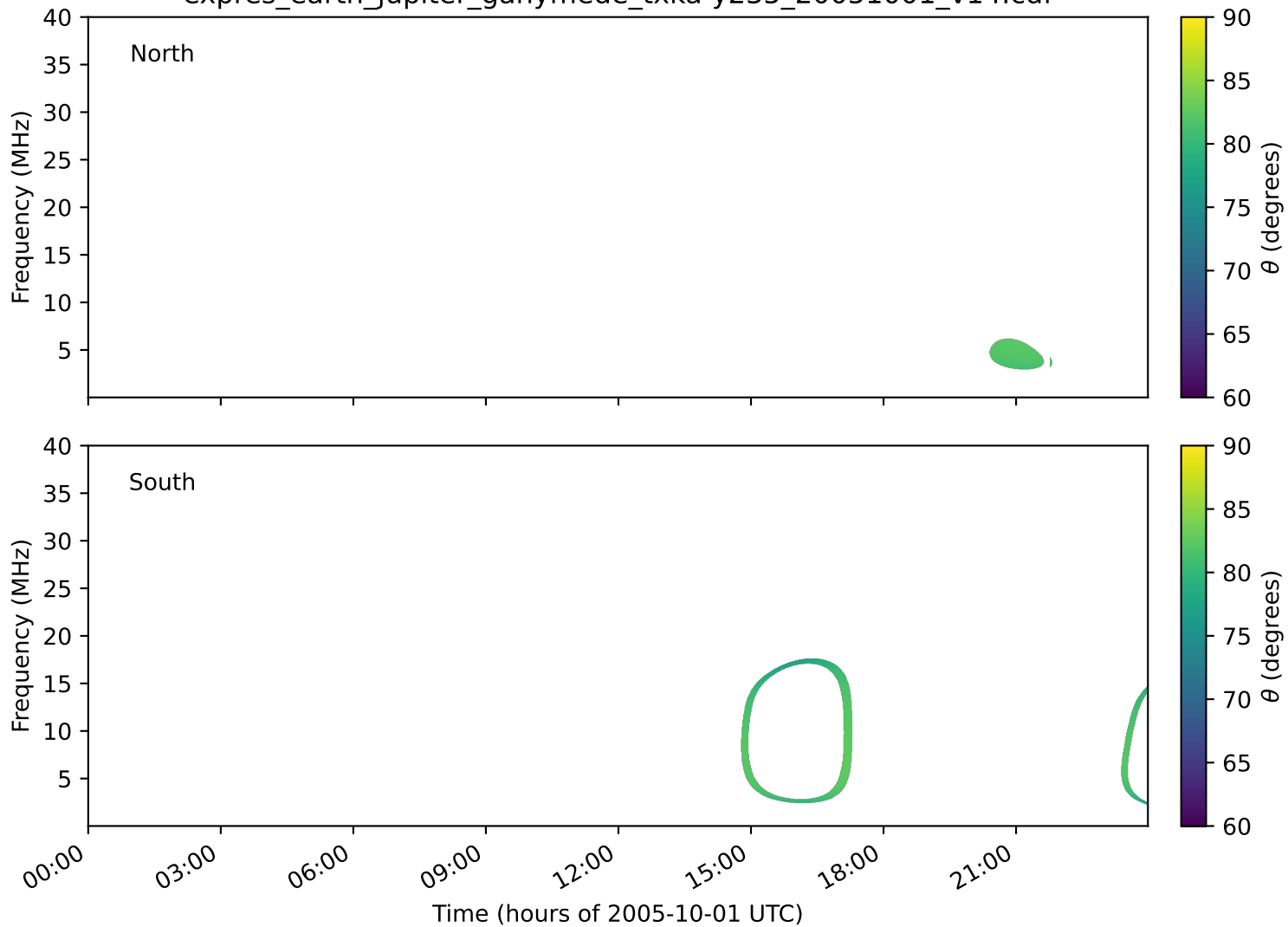
expres_earth_jupiter_ganymede_txka-y235_20051001_v14.cdf
