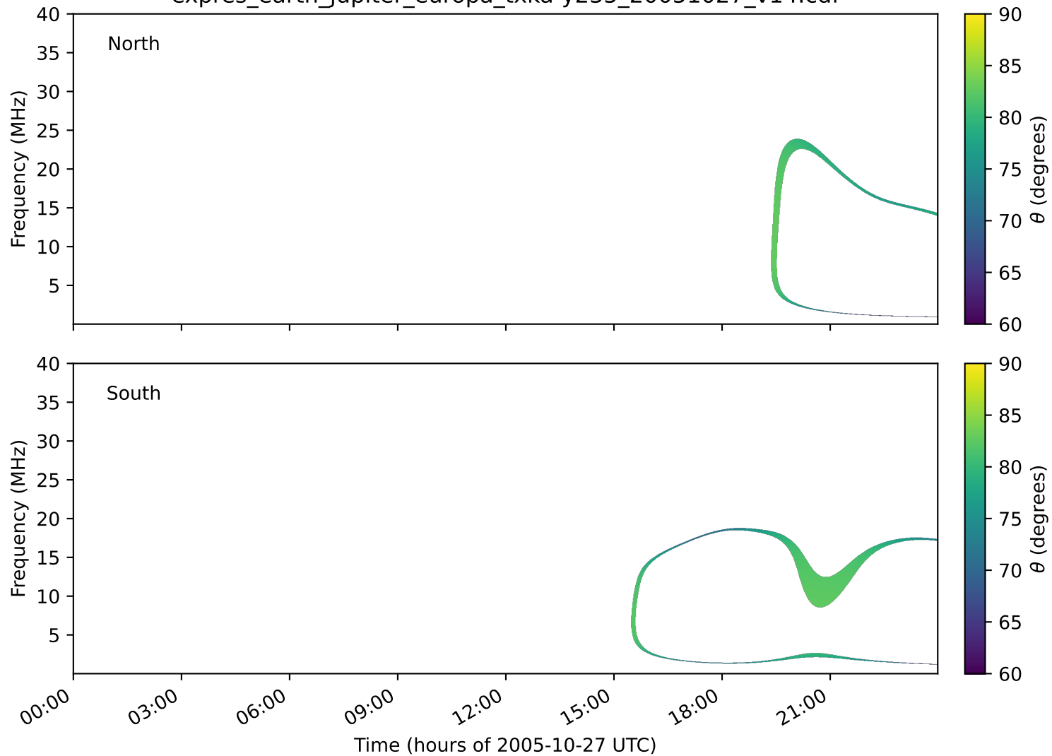
expres_earth_jupiter_europa_txka-y235_20051027_v14.cdf
