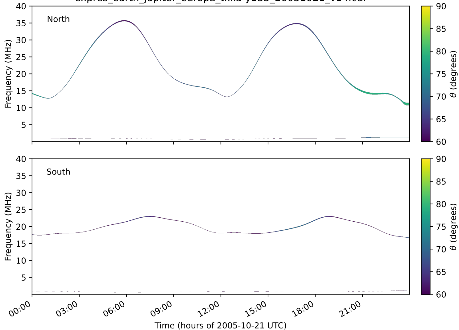
expres_earth_jupiter_europa_txka-y235_20051021_v14.cdf
