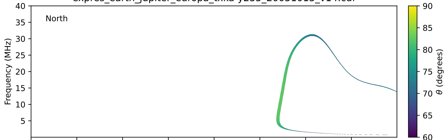
expres_earth_jupiter_europa_txka-y235_20051013_v14.cdf
