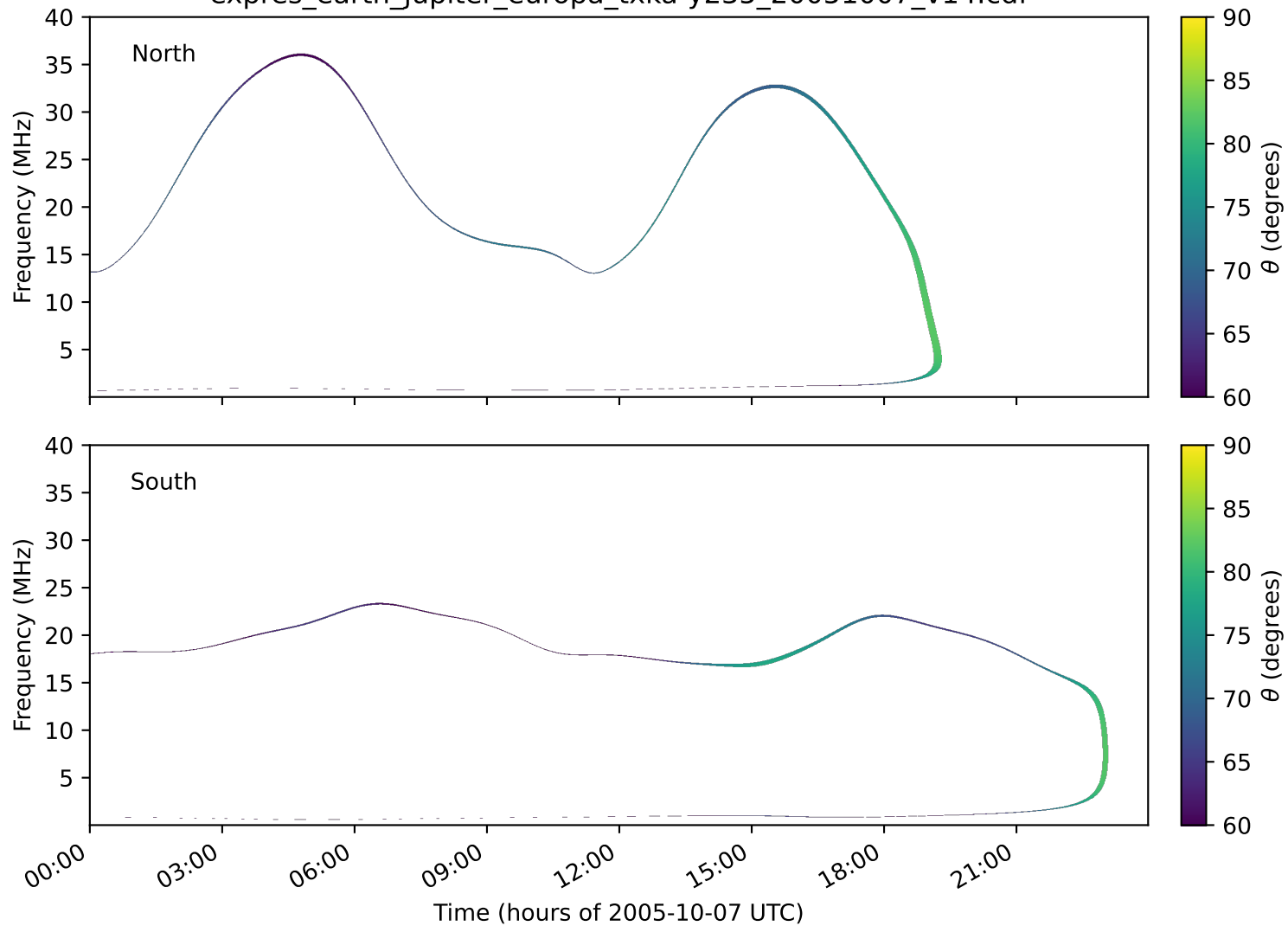
expres_earth_jupiter_europa_txka-y235_20051007_v14.cdf
