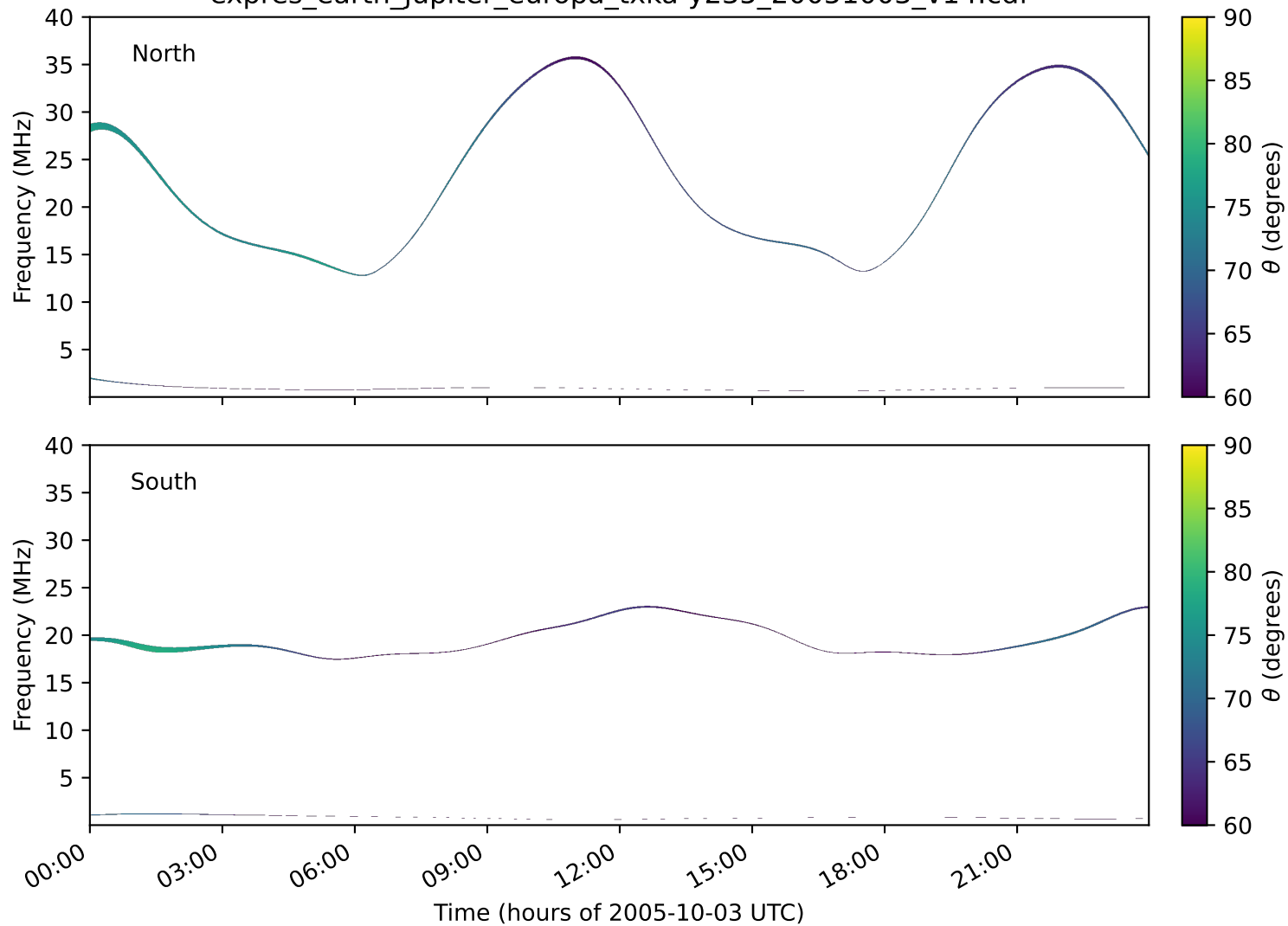
expres_earth_jupiter_europa_txka-y235_20051003_v14.cdf
