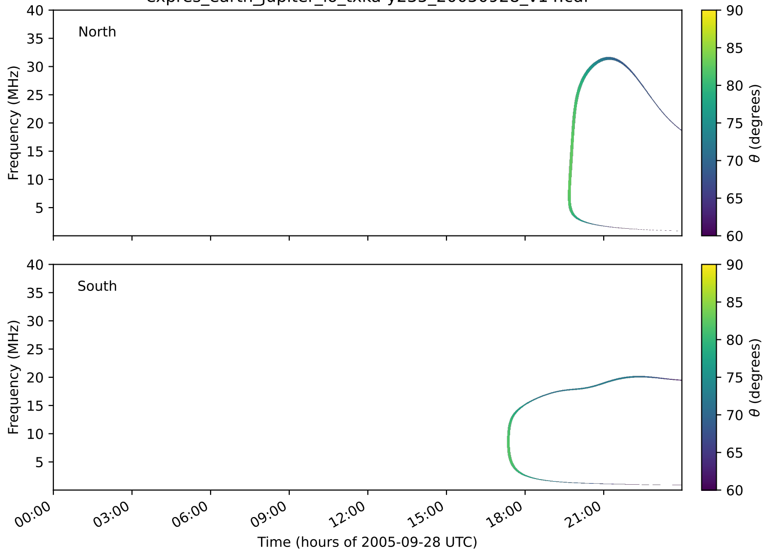
expres_earth_jupiter_io_txka-y235_20050928_v14.cdf
