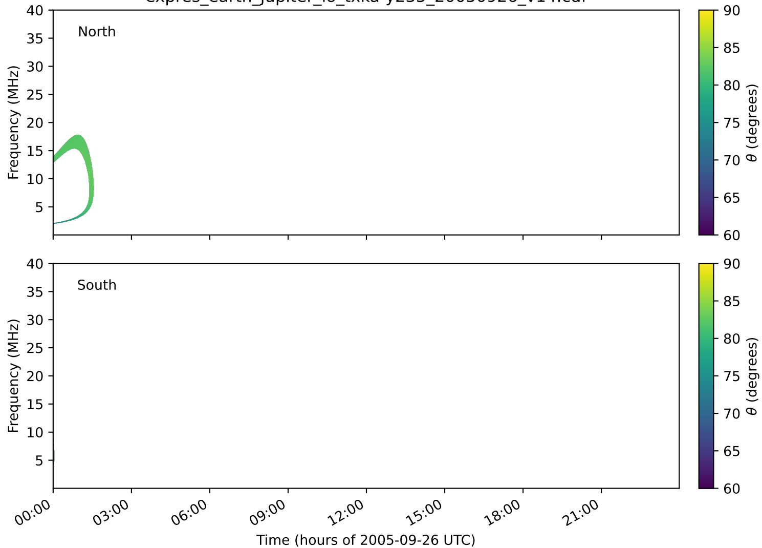
expres_earth_jupiter_io_txka-y235_20050926_v14.cdf
