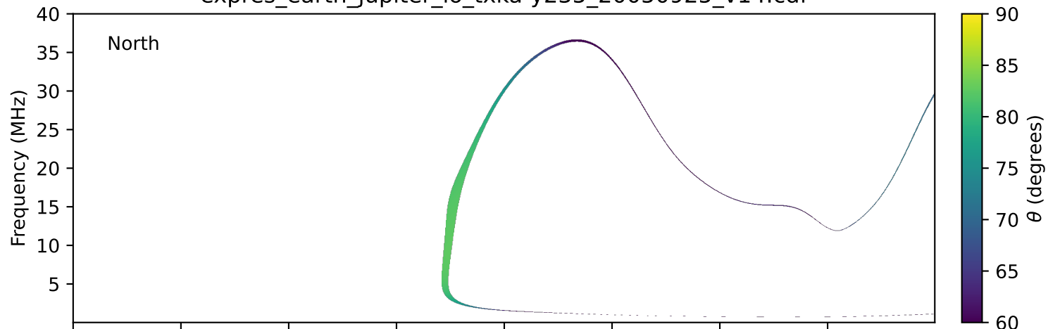
expres_earth_jupiter_io_txka-y235_20050925_v14.cdf
