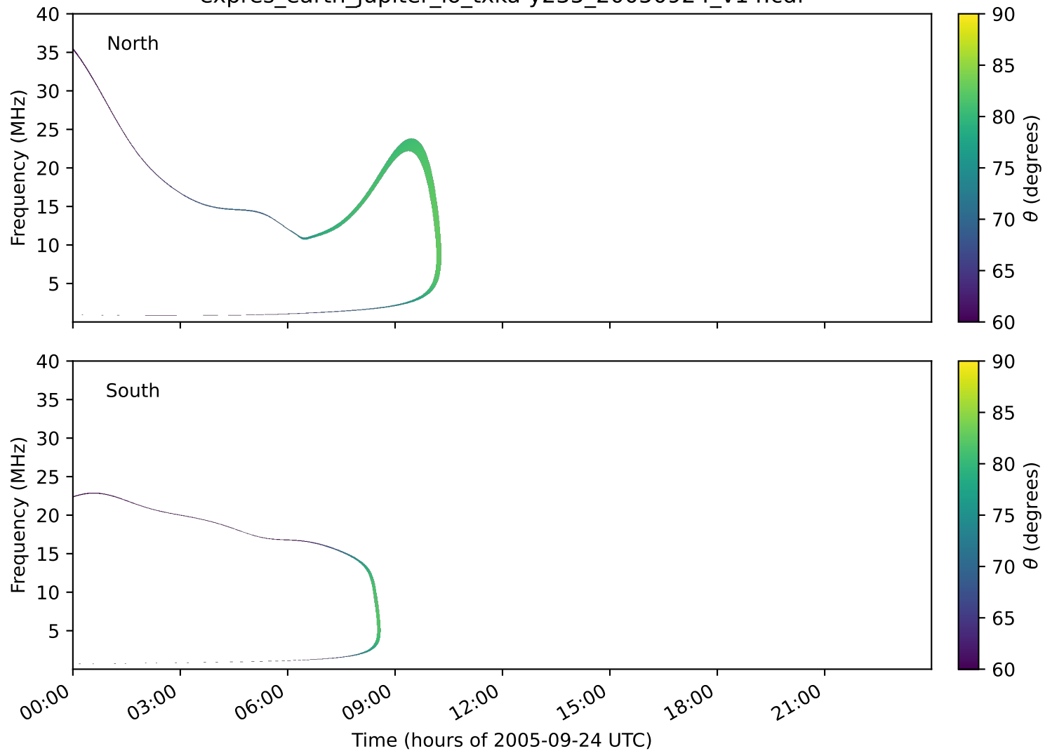
expres_earth_jupiter_io_txka-y235_20050924_v14.cdf
