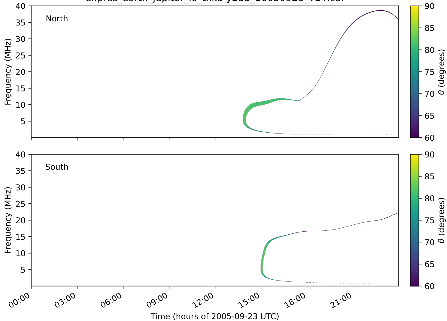
expres_earth_jupiter_io_txka-y235_20050923_v14.cdf
