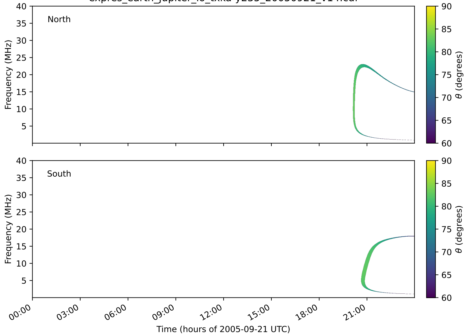
expres_earth_jupiter_io_txka-y235_20050921_v14.cdf
