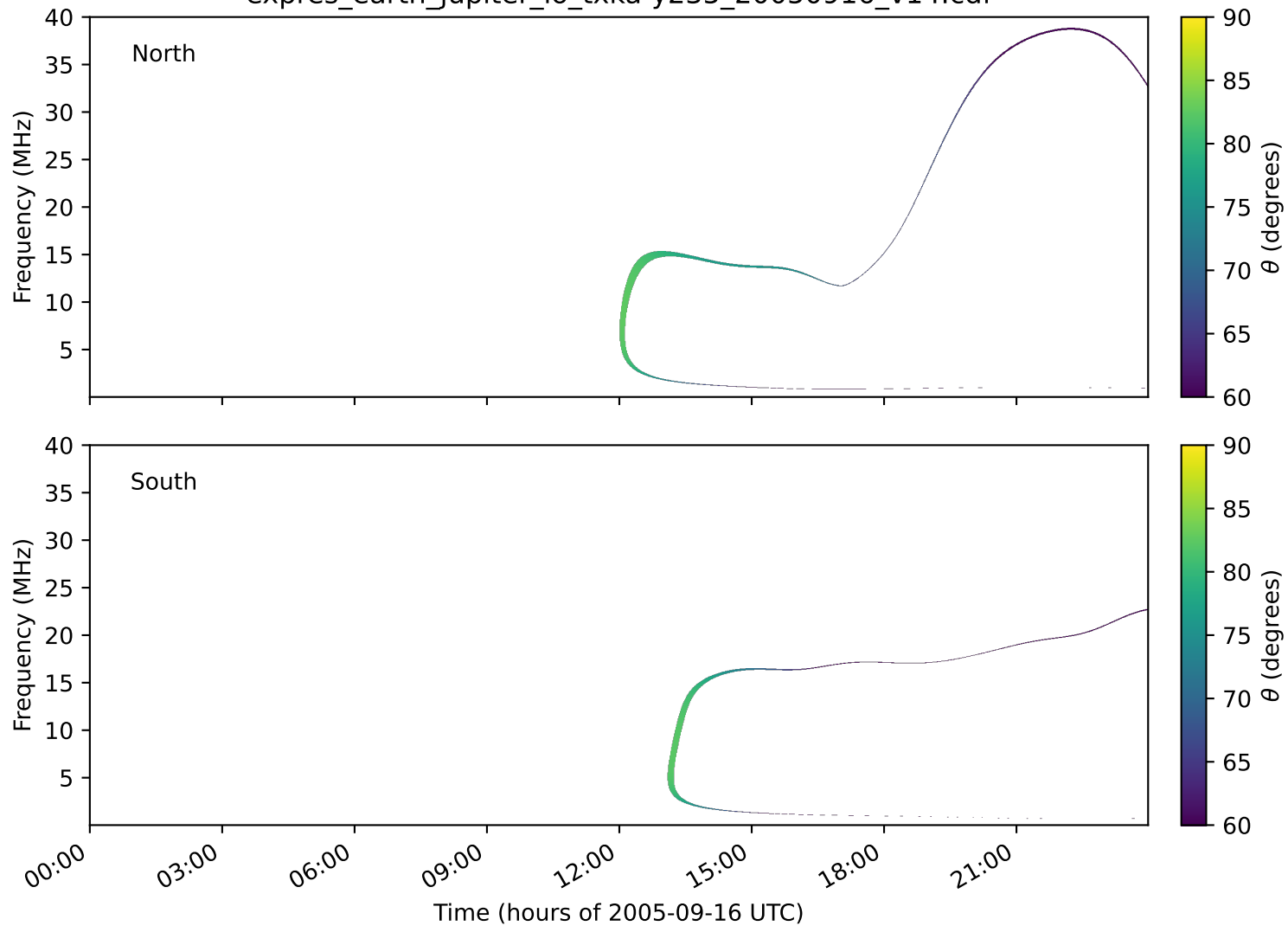
expres_earth_jupiter_io_txka-y235_20050916_v14.cdf
