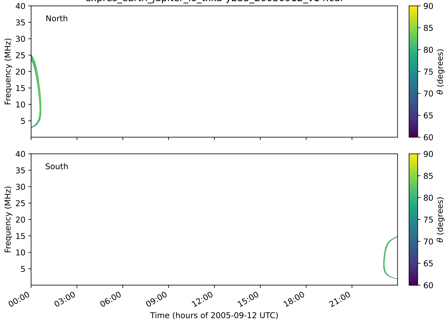
expres_earth_jupiter_io_txka-y235_20050912_v14.cdf
