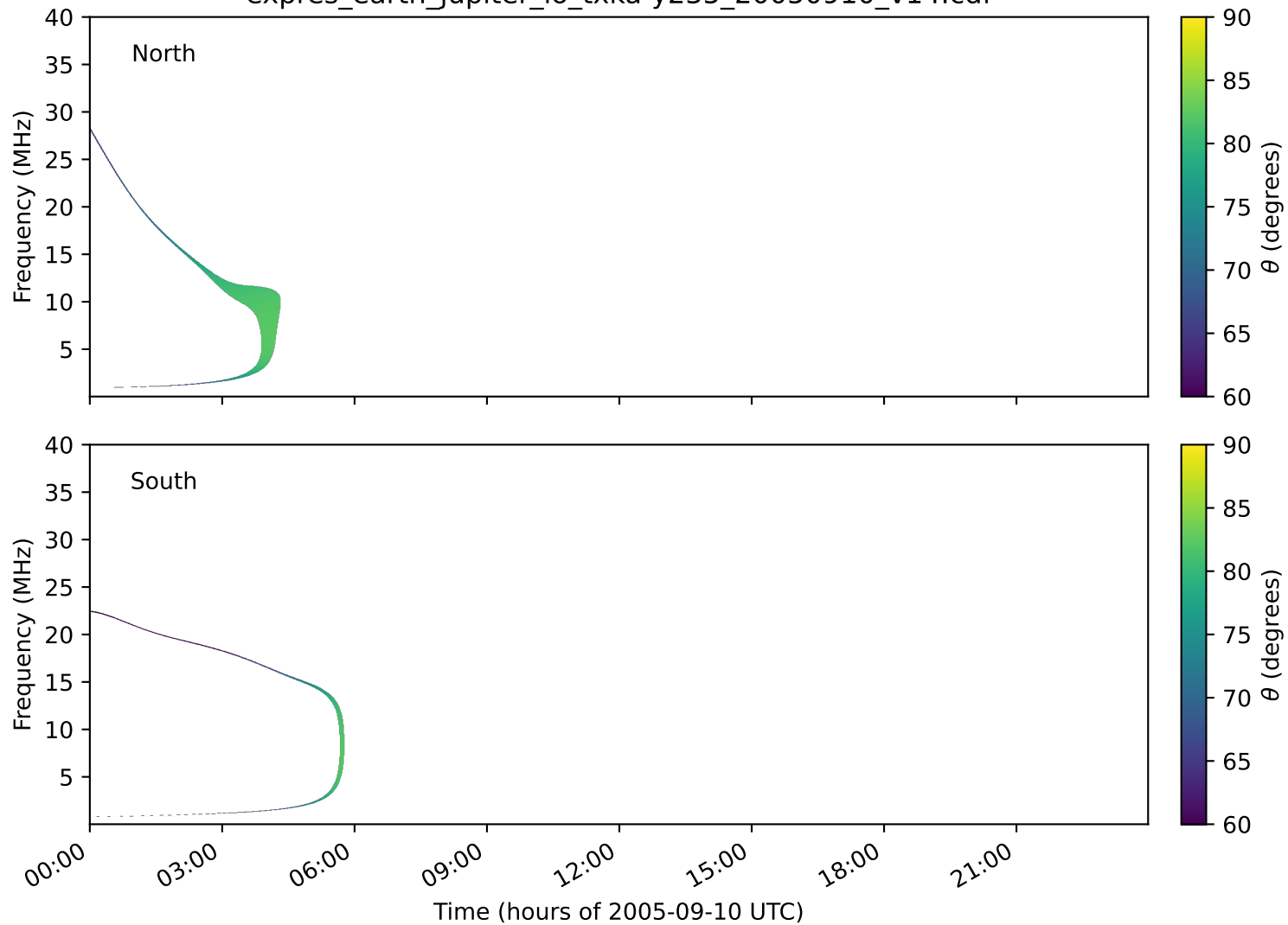
expres_earth_jupiter_io_txka-y235_20050910_v14.cdf
