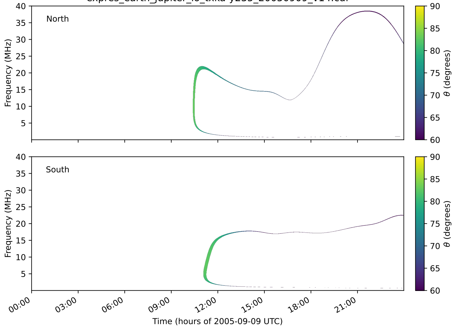
expres_earth_jupiter_io_txka-y235_20050909_v14.cdf
