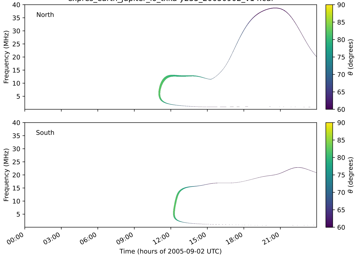
expres_earth_jupiter_io_txka-y235_20050902_v14.cdf
