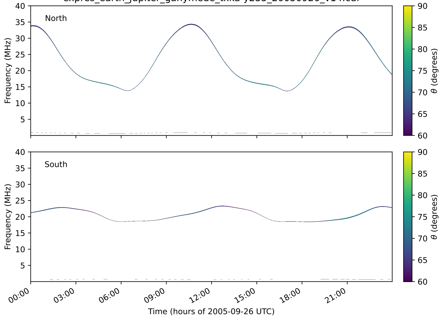
expres_earth_jupiter_ganymede_txka-y235_20050926_v14.cdf
