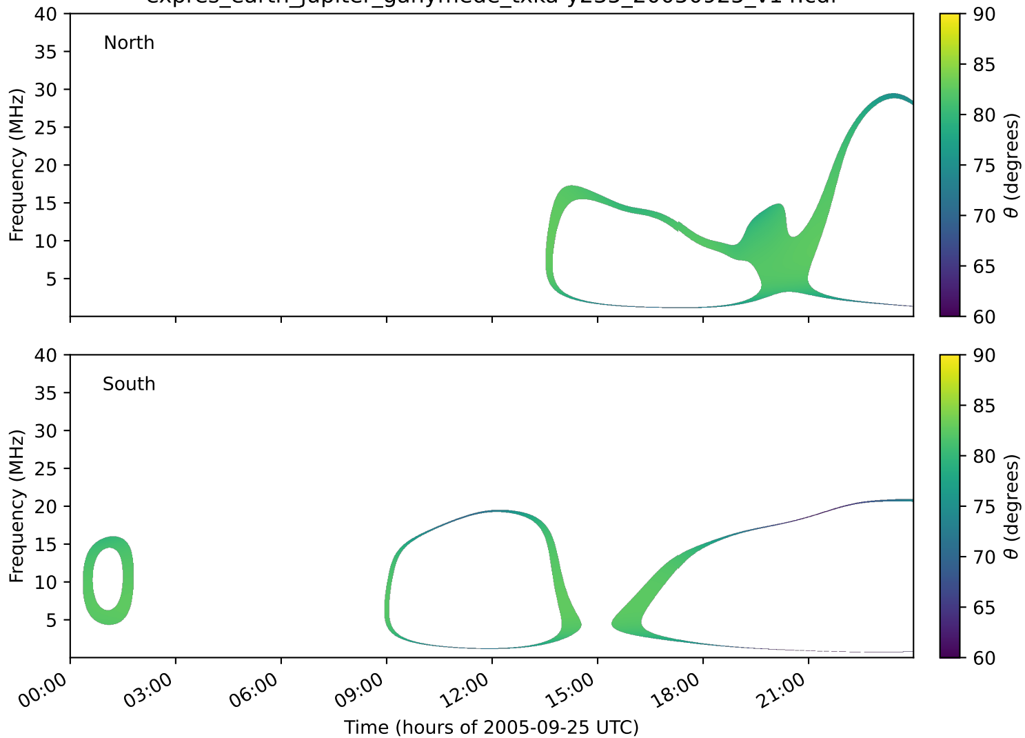
expres_earth_jupiter_ganymede_txka-y235_20050925_v14.cdf
