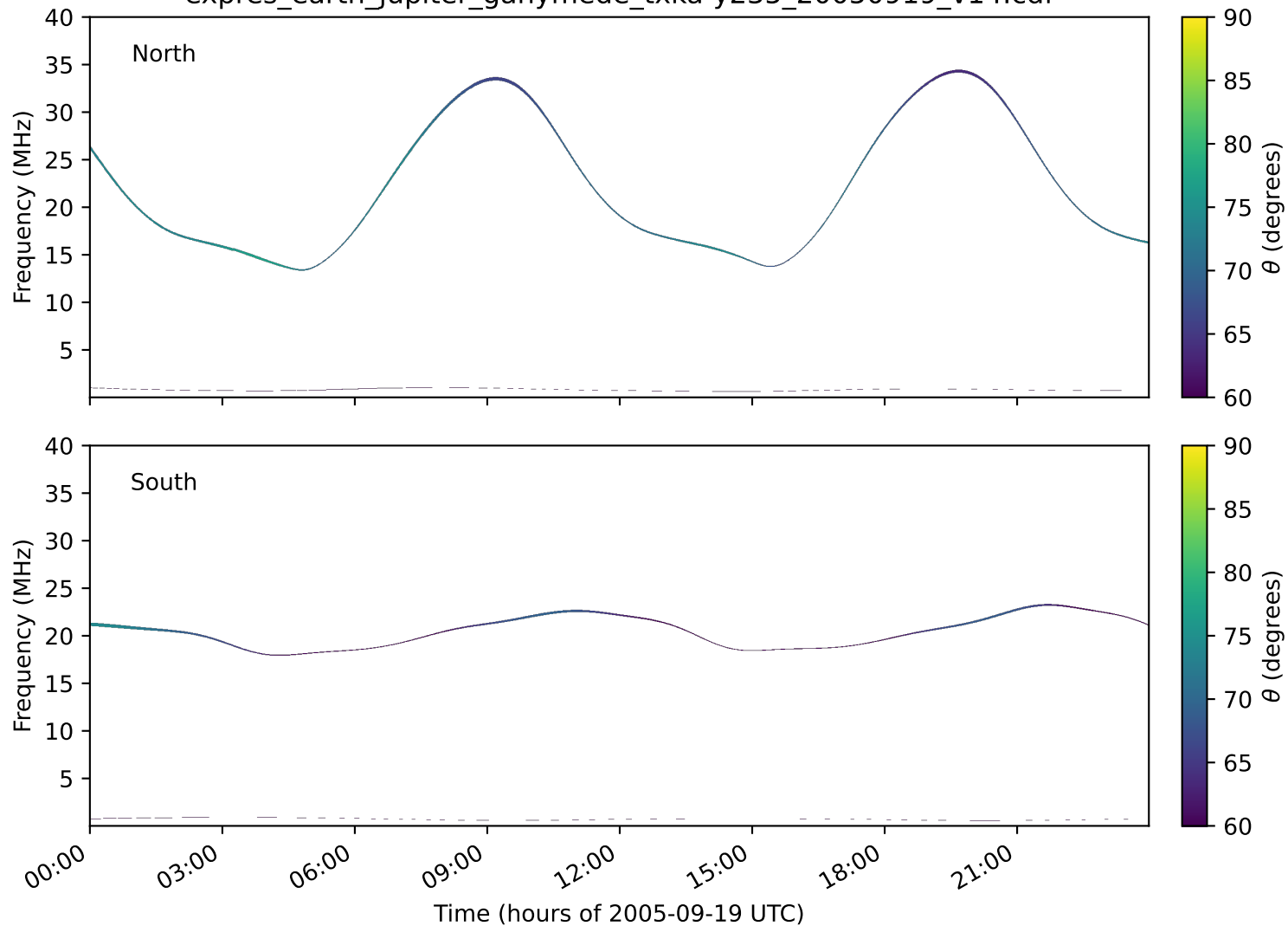
expres_earth_jupiter_ganymede_txka-y235_20050919_v14.cdf
