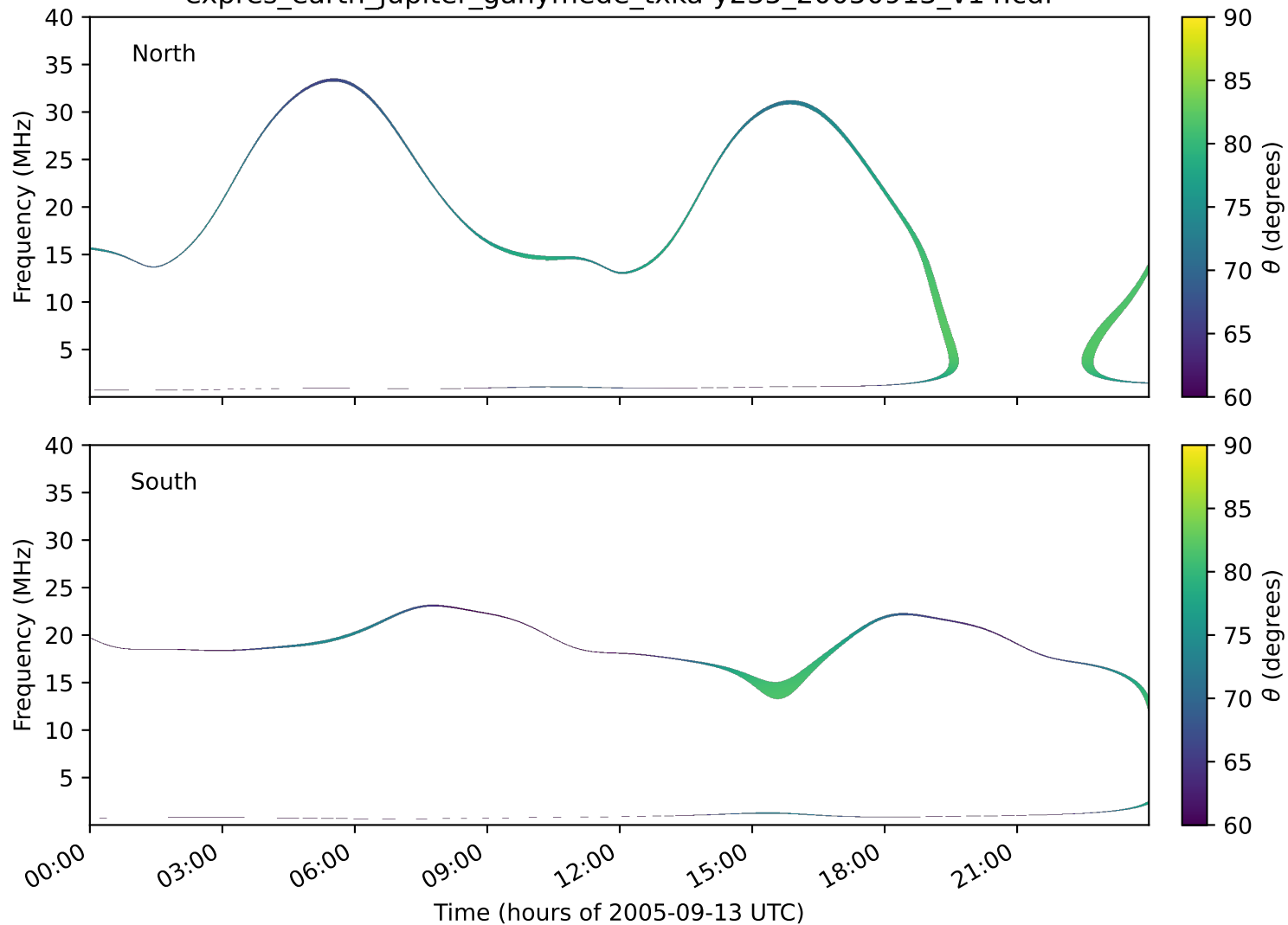
expres_earth_jupiter_ganymede_txka-y235_20050913_v14.cdf
