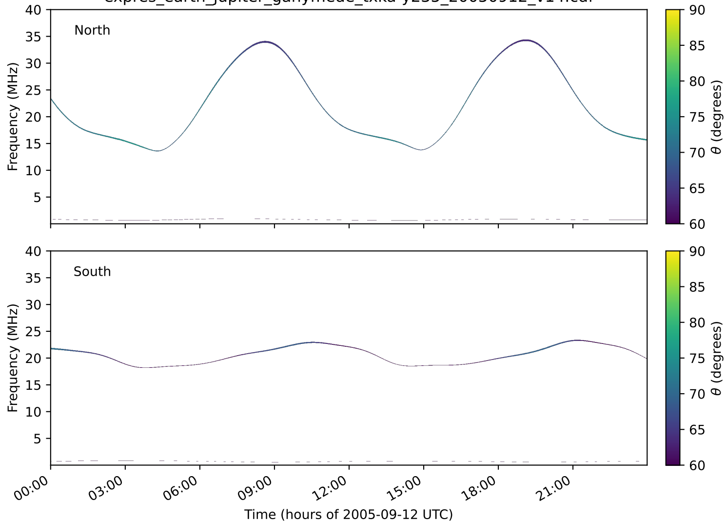
expres_earth_jupiter_ganymede_txka-y235_20050912_v14.cdf
