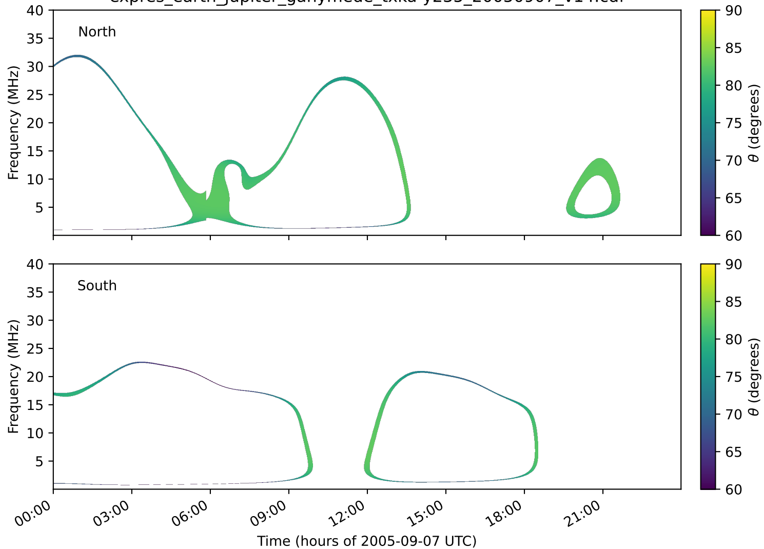
expres_earth_jupiter_ganymede_txka-y235_20050907_v14.cdf
