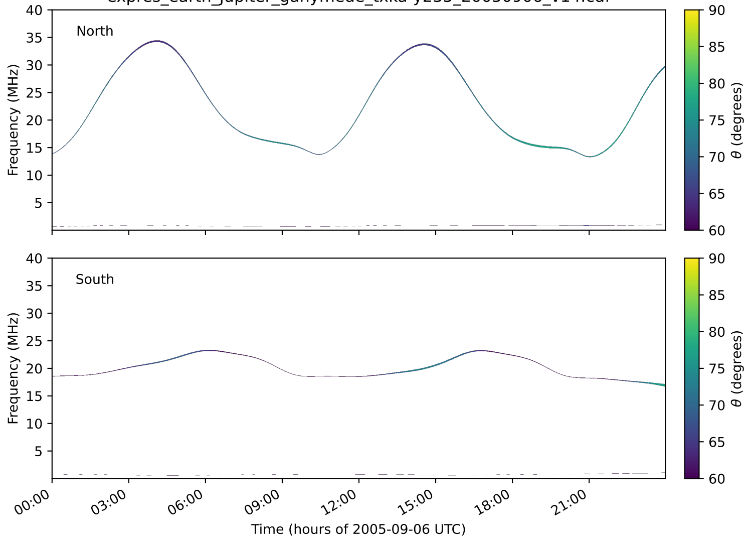
expres_earth_jupiter_ganymede_txka-y235_20050906_v14.cdf
