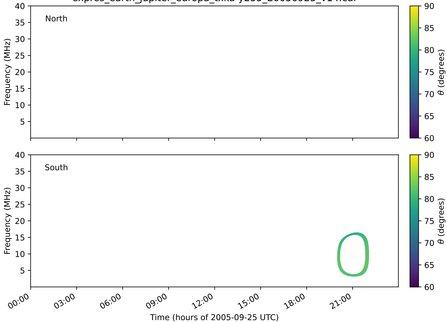
expres_earth_jupiter_europa_txka-y235_20050925_v14.cdf
