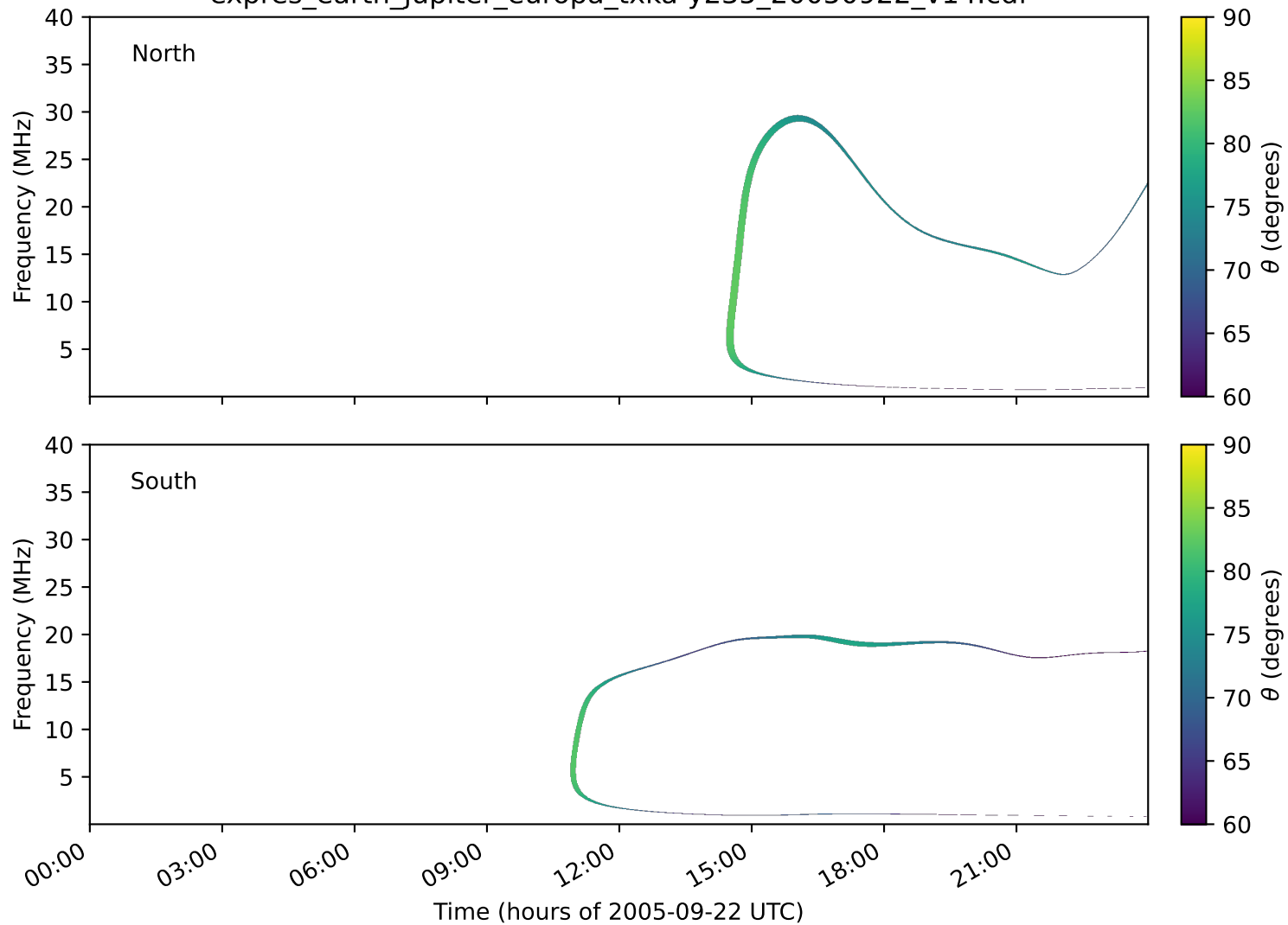
expres_earth_jupiter_europa_txka-y235_20050922_v14.cdf
