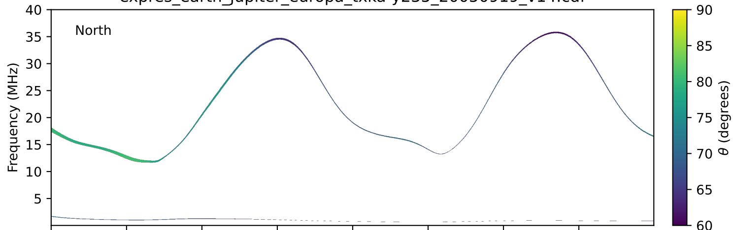
expres_earth_jupiter_europa_txka-y235_20050919_v14.cdf
